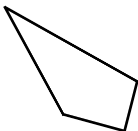
Irregular quadrilateral
